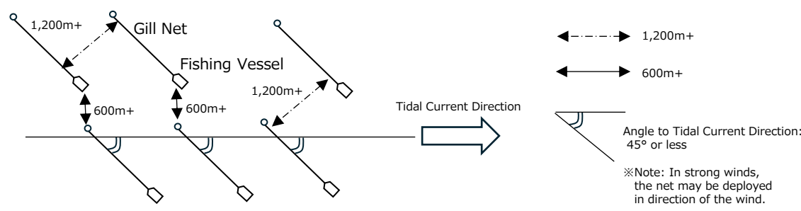
(Fig.2) Direction of Gill Net Deployment
